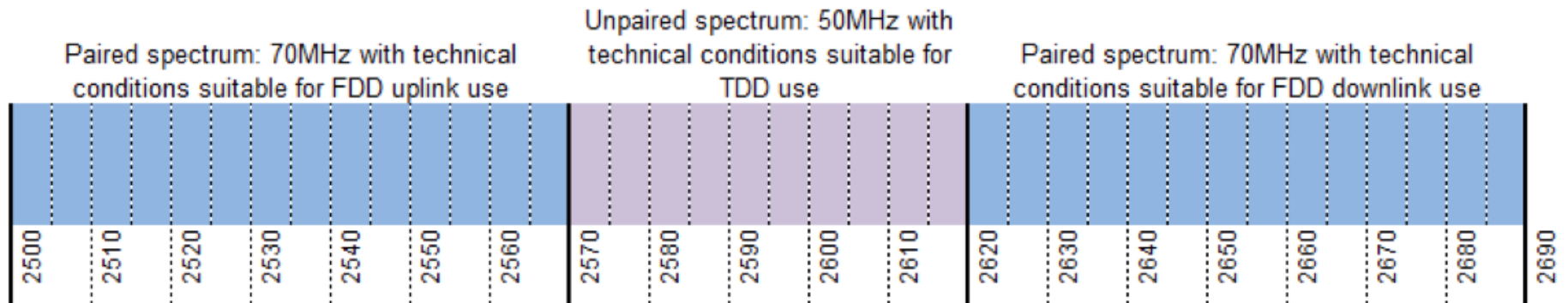
Figure 4.3: 2.6 GHz band plan
