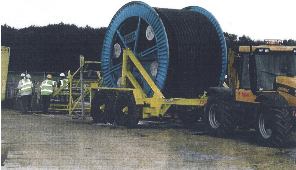
Figure 38 – Cable drum carrying trailer
